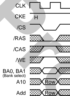
Row Address Strobe and Bank Activate Command
