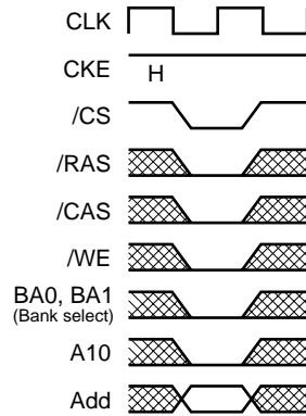
Mode Register Set Command
