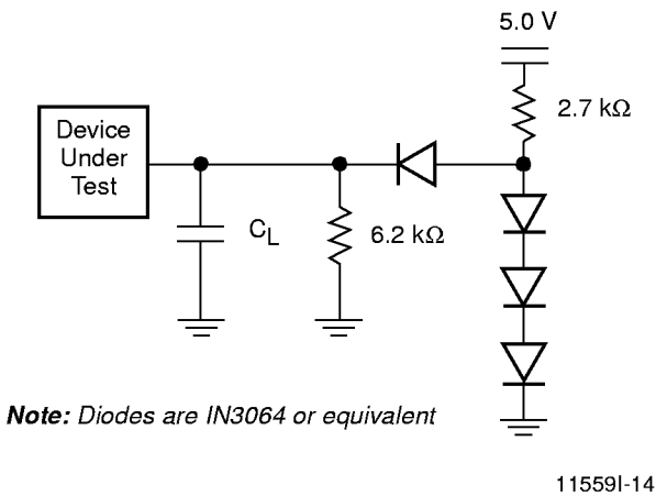
Figure 6. Test Setup
