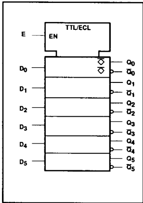
SIMPLIFIED SCHEMATIC
