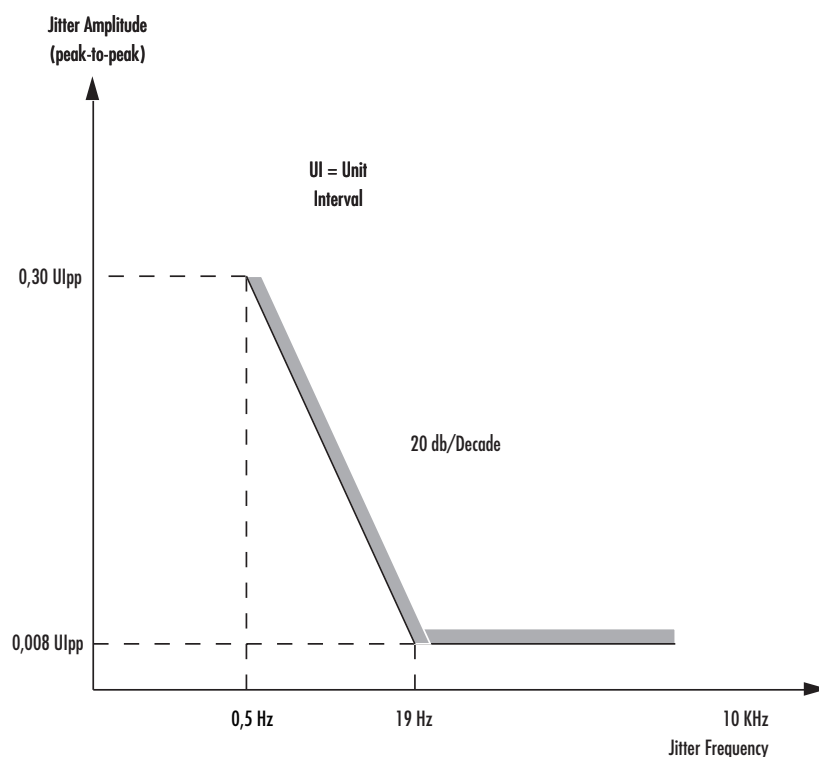
Fig.6: Range of Admissible Sinusoidal Input Jitter
