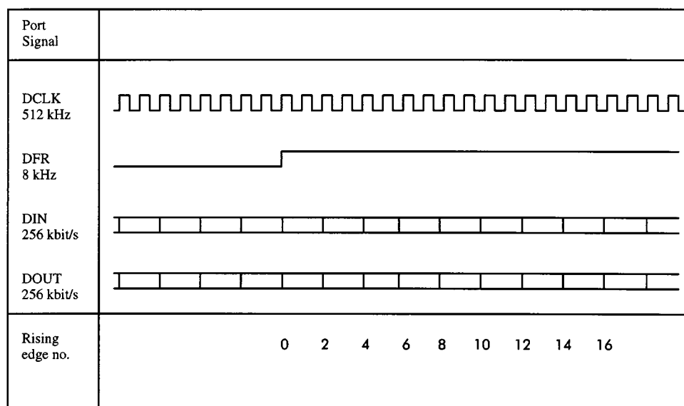
Fig.12: Timing of Data and Clocks at the GCI Interface
