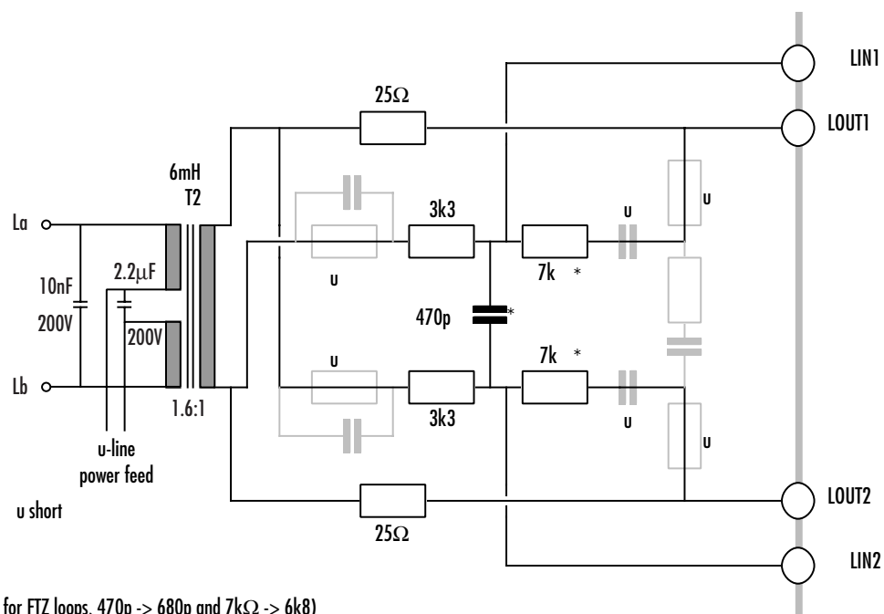
Fig.5a: 4B3T - Recommended Hybrid Component Configuration, using same PCB layout as 2B1Q,
