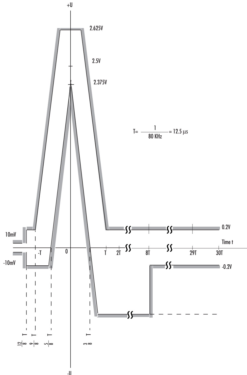
Fig.8: Single Pulse Mask
