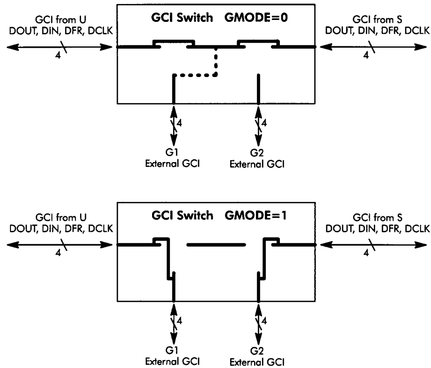
Fig.15: External GCI Interface
