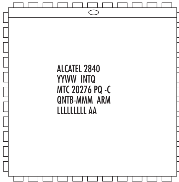
Fig.23: Device Marking-PQ Order number MTC-20276 PQ-I or C
