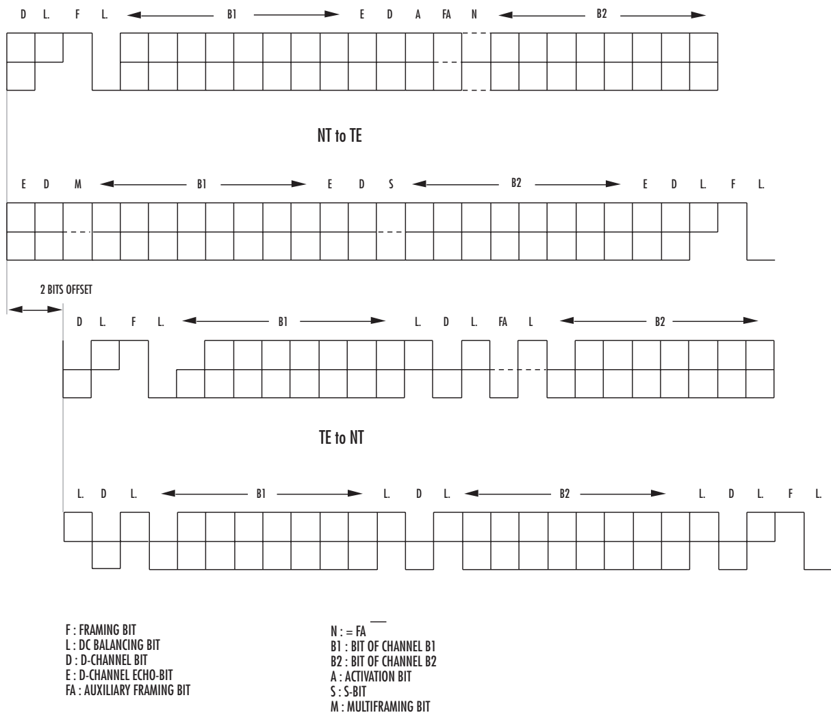
Fig.19: So-Frame Format
