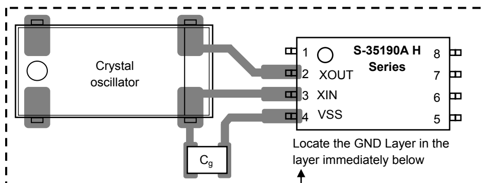
Figure 45 Connection Diagram 2
