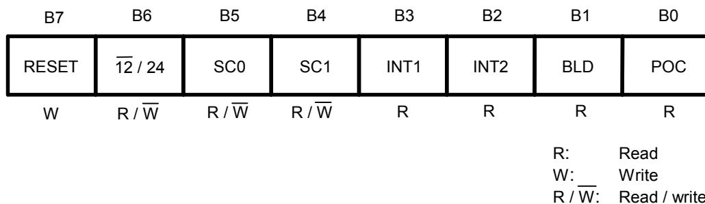
Figure 14 Status Register 1
