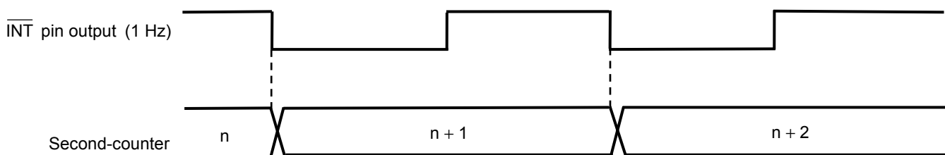
Figure 19 1 Hz Clock Output and Second-counter
