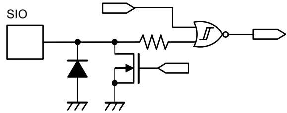
Figure 5 SIO Pin
