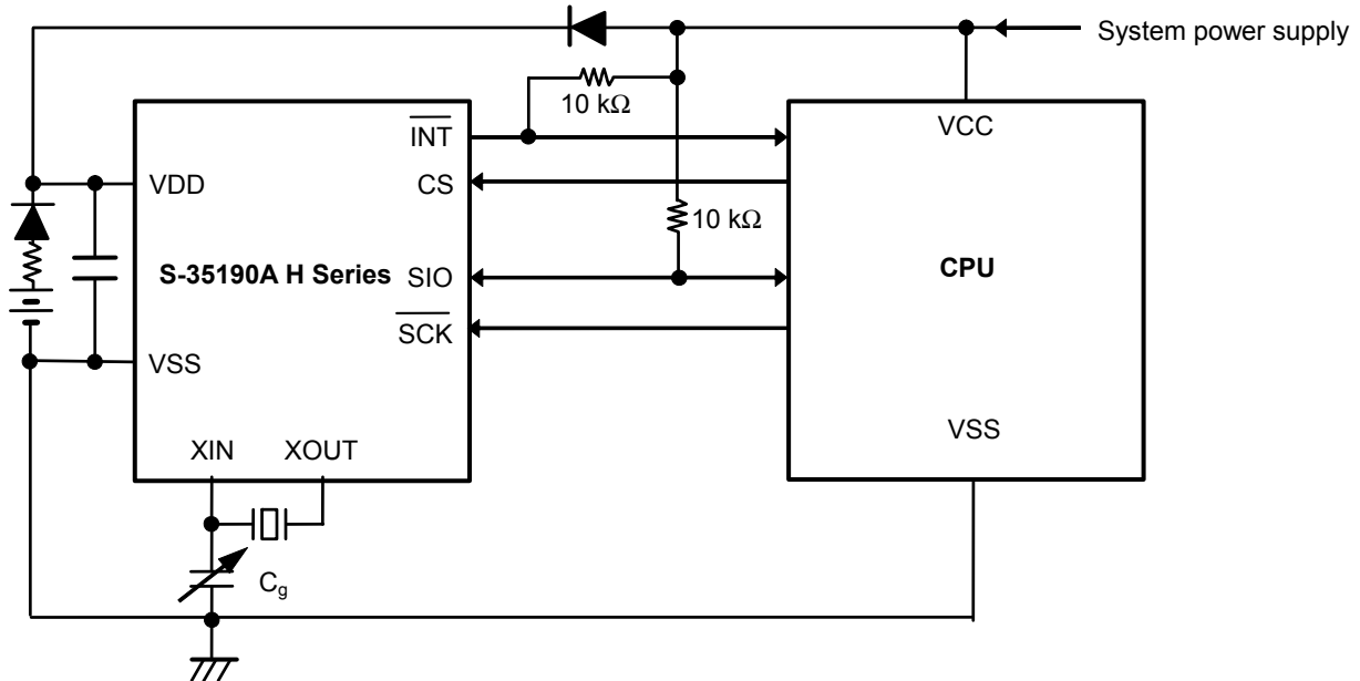
Figure 42 Application Circuit 1
