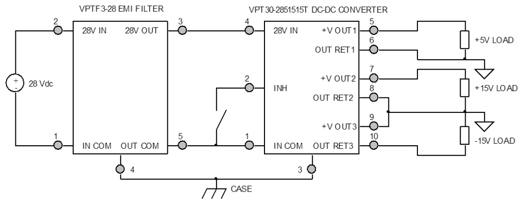
(Shown with optional VPTF3-28 EMI filter, recommended for input voltages > 13V, and optional negative output configuration.)
