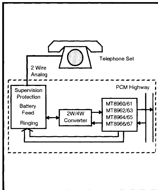
Figure 6 - Typical Line Termination
