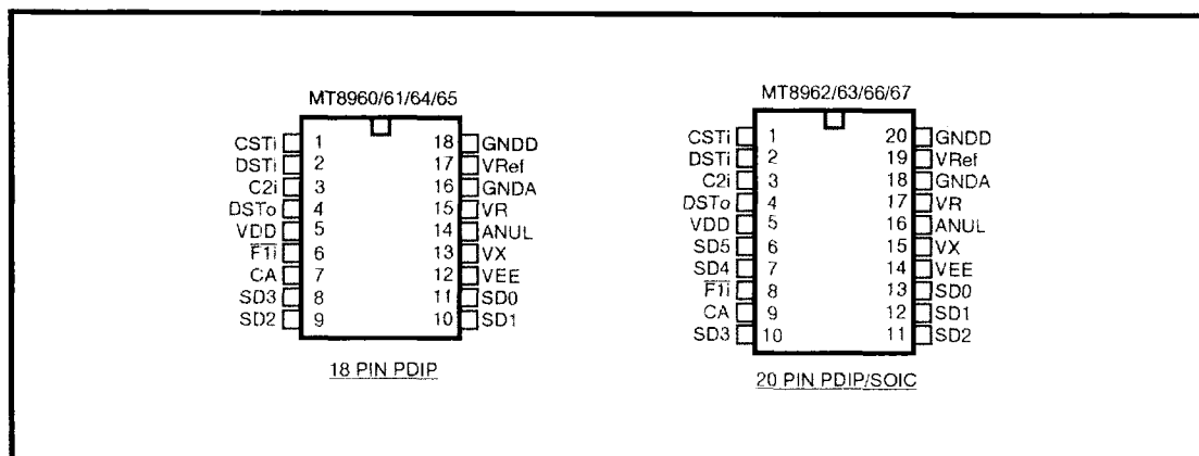
Figure 2 - Pin Connections
