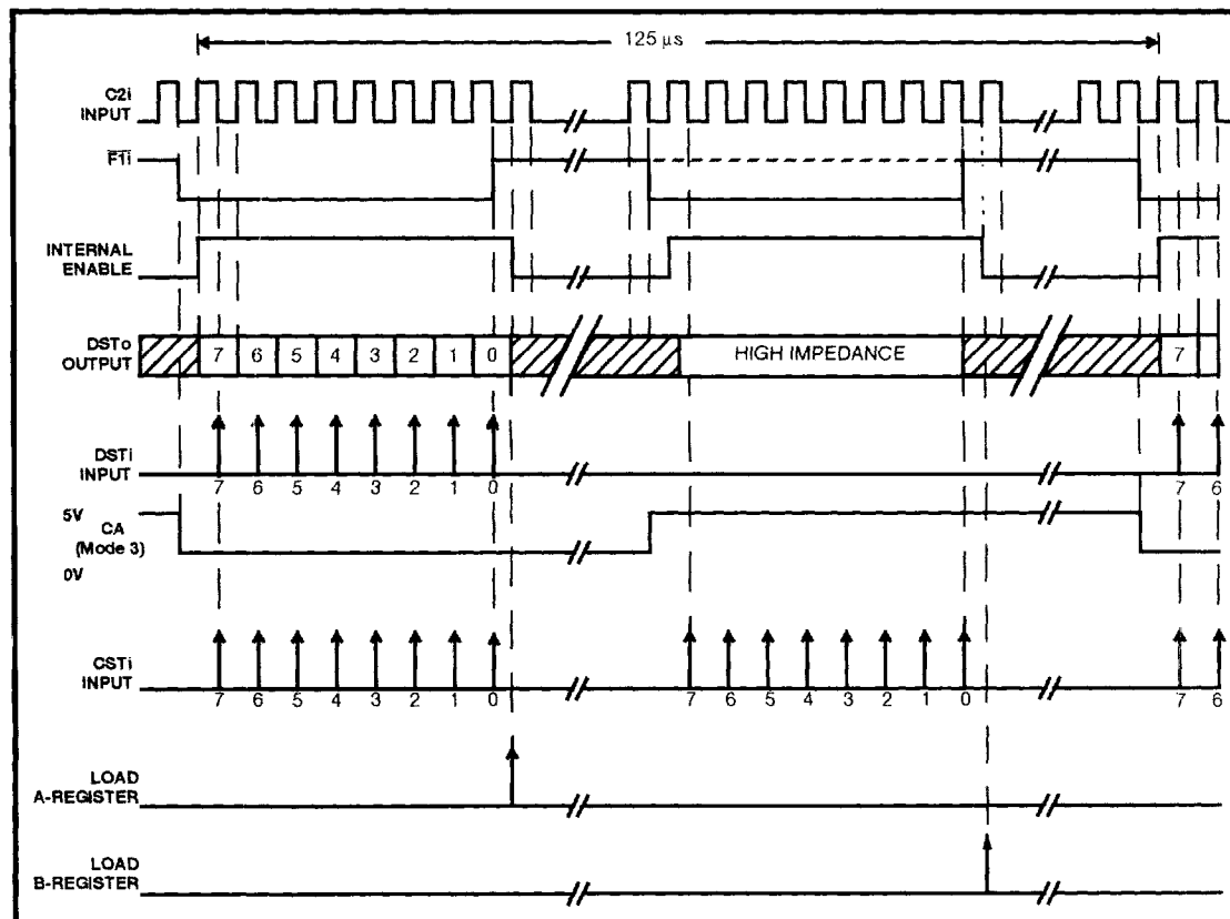
Figure 9a - Timing Diagram - 125 \mu\text{s} Frame Period
