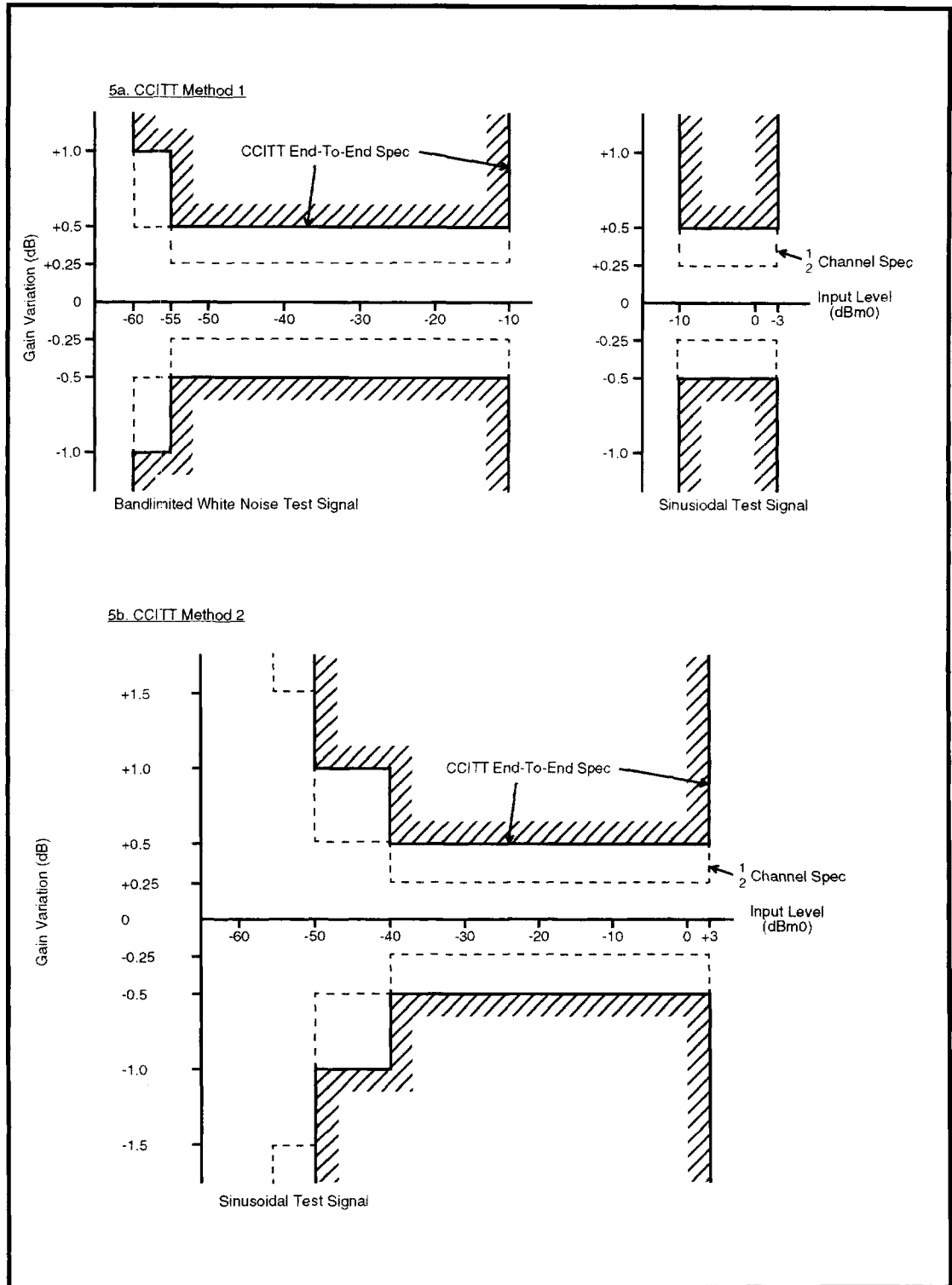
Figure 12 - Variation of Gain With Input Level
