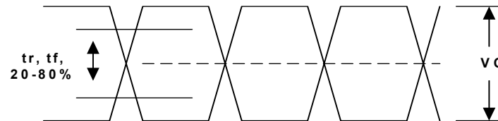
Figure 3. ECL/LVPECL Output
