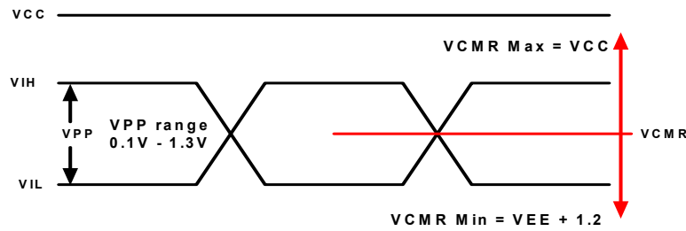
Figure 1. PECL/ECL Input Waveform Definitions
