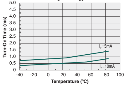
Typical Turn-On Time vs. Temperature ( I_L=70mA_{DC} )
