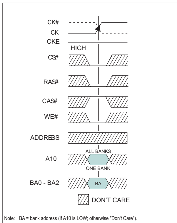
FIGURE 13 – PRECHARGE COMMAND
