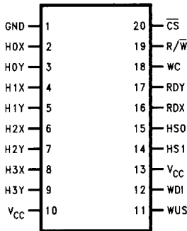
FIGURE 2. Connection Diagram
