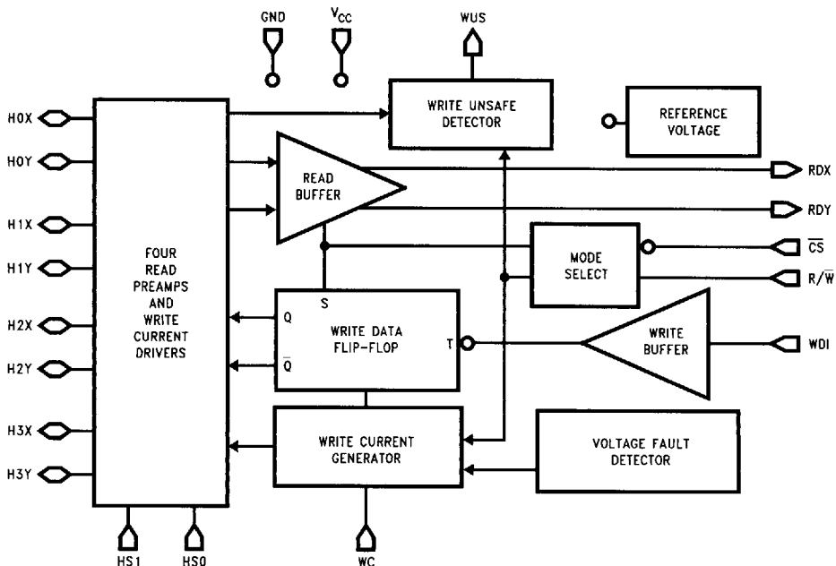
FIGURE 1. Circuit Block Diagram
