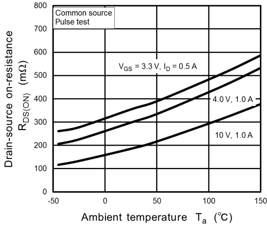
Fig. 7.7 R_{DS(ON)} - T_a
