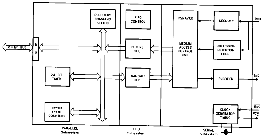
Figure 1. 82590 Block Diagram
