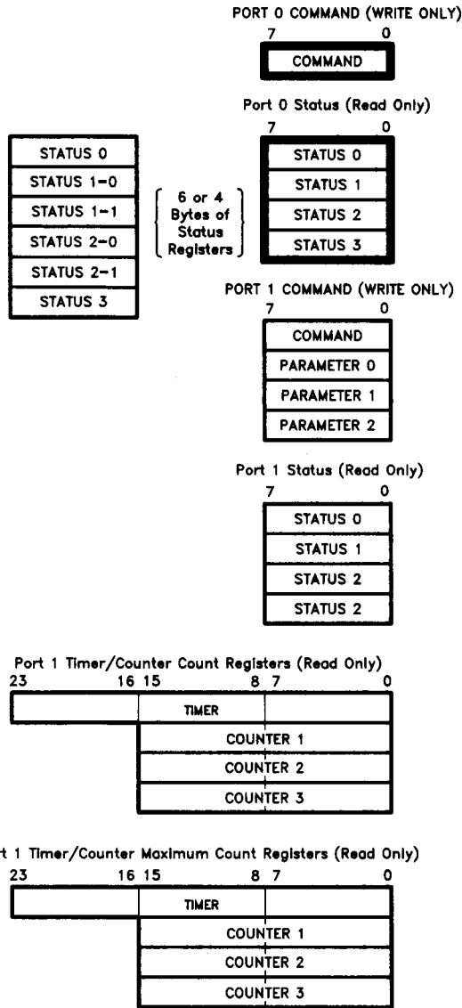
Figure 4. Programming Model—Directly Accessible Registers (Accessible Through 8-Bit I/O Port(s))
