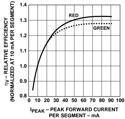
Figure 4. Relative Efficiency (Luminous Intensity Per Unit Current Per Dot) vs. Peak Current Per Dot.
