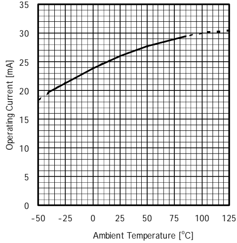
Operating Current vs. Ambient Temperature IEE V+=7V V=-7V
