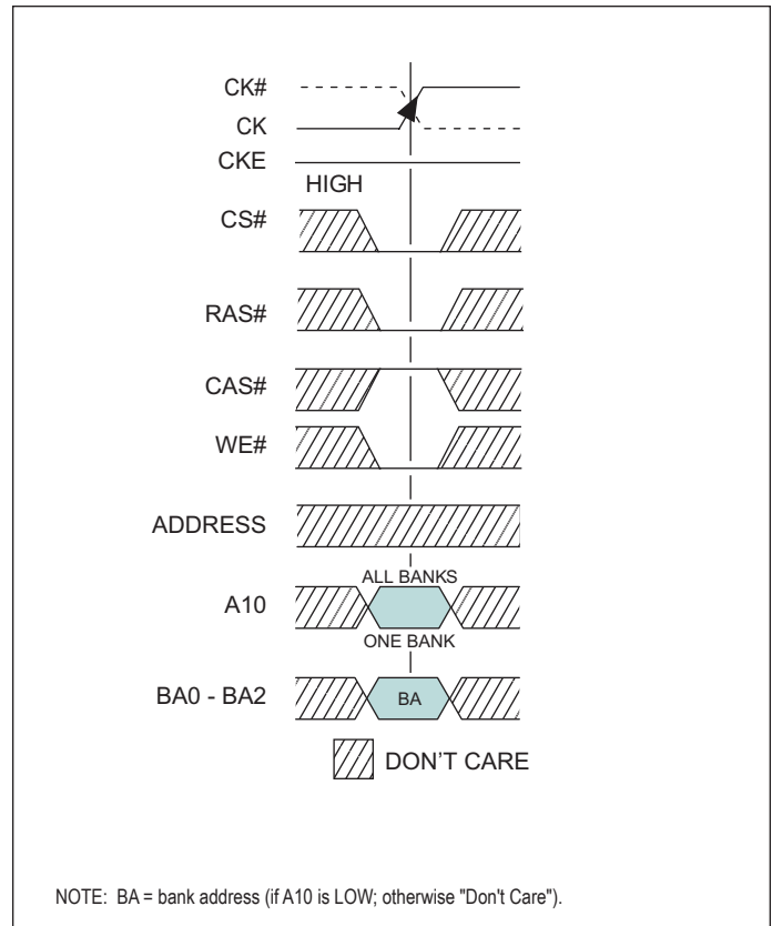
FIGURE 13 – PRECHARGE COMMAND
