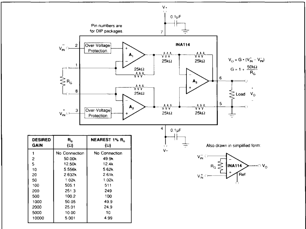
FIGURE 1. Basic Connections.
