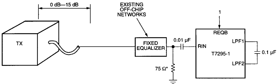
Figure 4. Receiver Configurations
