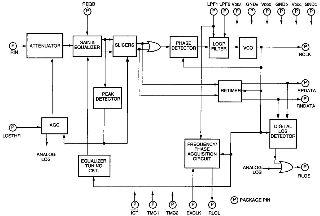
Figure 1. Block Diagram
