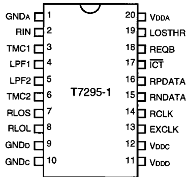
Figure 2. Pin Layout
