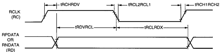
Figure 9. Timing Diagram for System Interface
