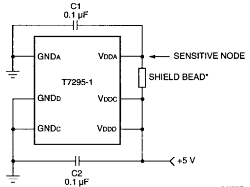
Figure 8. Recommended Power Supply Bypassing Network
