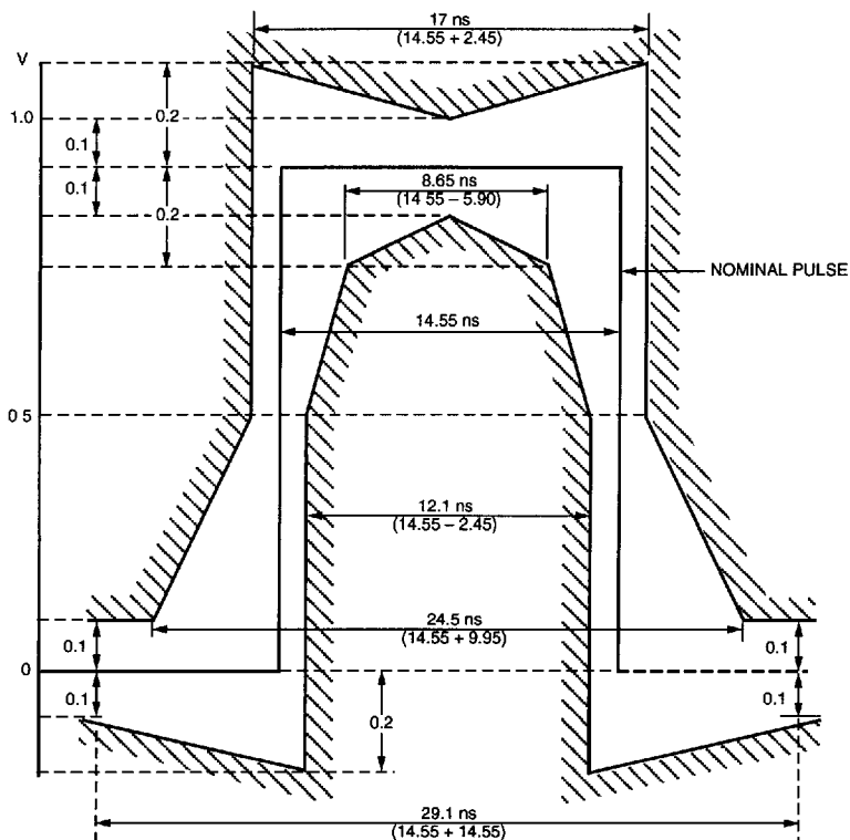
Figure 5. Isolated E3 Pulse Template
