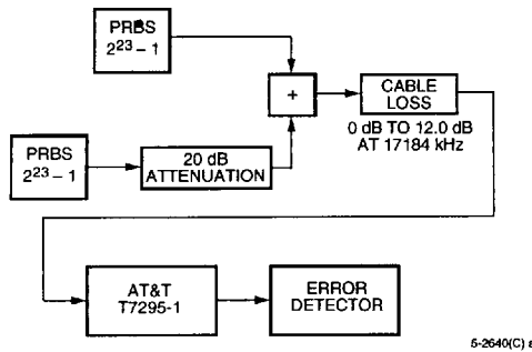
Figure 7. Test Setup for Interference Immunity
