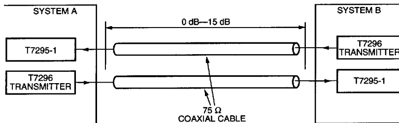
Figure 3. Application Diagram
