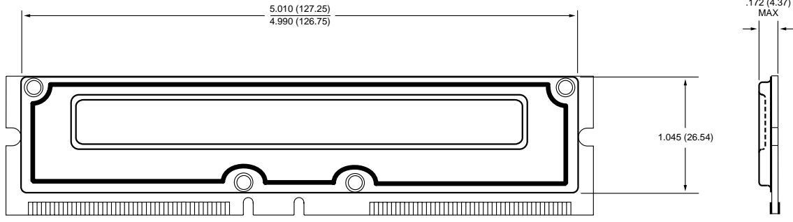
FRONT VIEW WITH HEAT SPREADER
