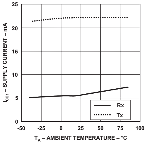
Figure 1. V_{CC1} supply current vs. temperature.
