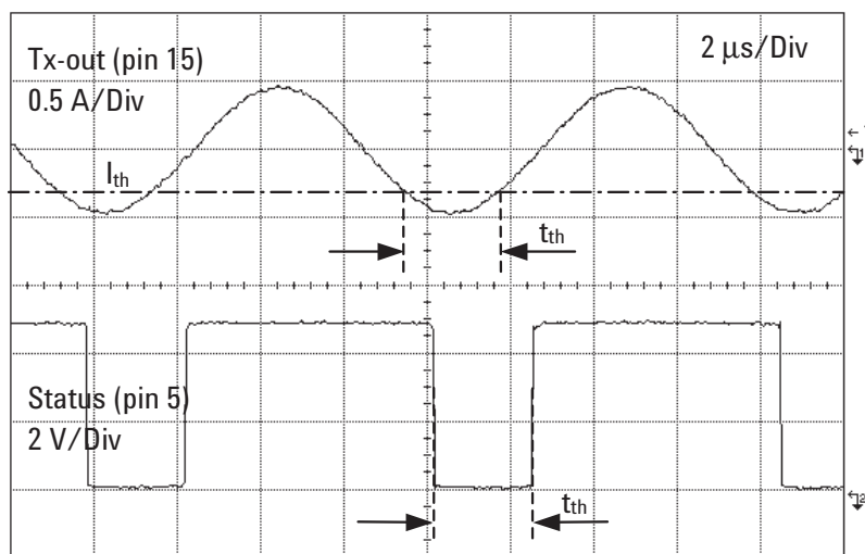
Figure 21. Transmit output load detection.
