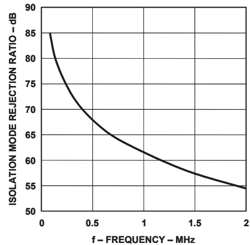
Figure 6. Isolation mode rejection ratio vs. frequency.
