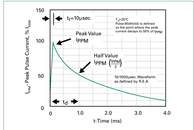
Figure 4 - Pulse Waveform
