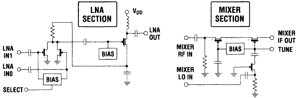
Simplified Circuit Schematic
