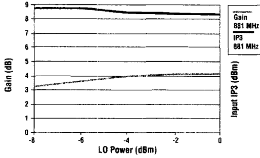
Gain and Input IP3 vs. LO Power
