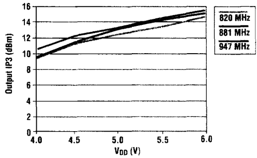
IP_3 vs. V_{DD} vs. Frequency
