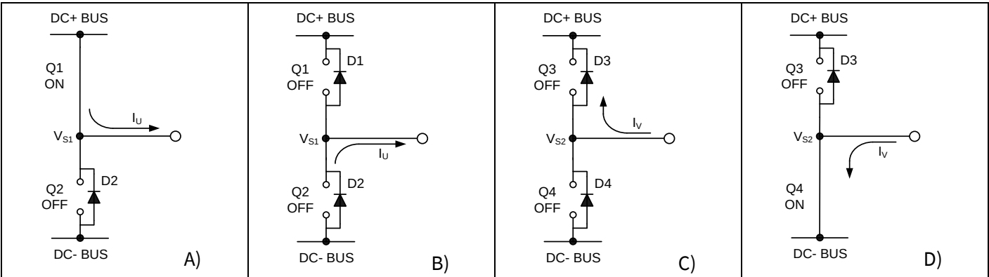
Figure 23 A) Q1 conducting B) D2 conducting C) D3 conducting D) Q4 conducting
