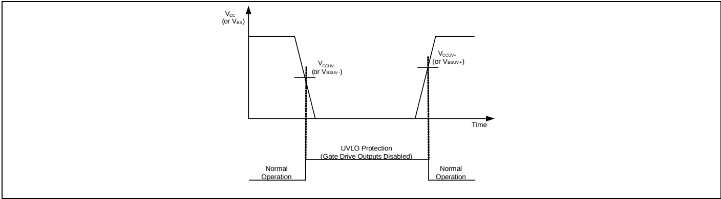
Figure 13 UVLO protection
