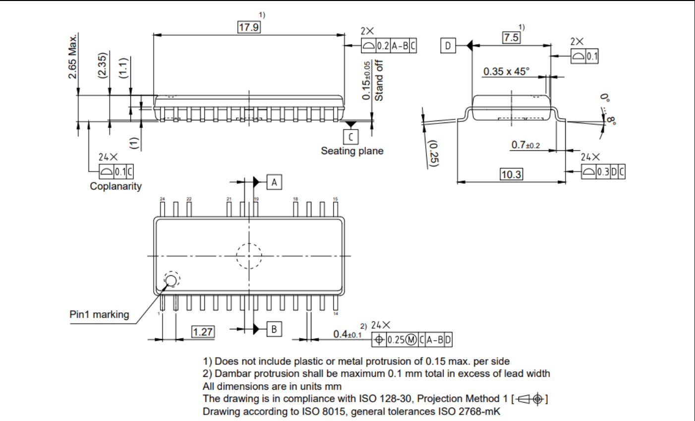
Figure 29 Package outline
