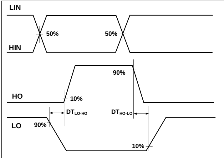
Figure 10 Dead Time Definitions
