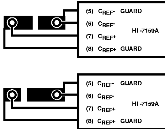
FIGURE 10. TYPICAL GUARD RING LAYOUT
