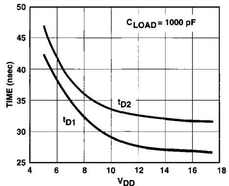
Propagation Delay vs. Supply Voltage
