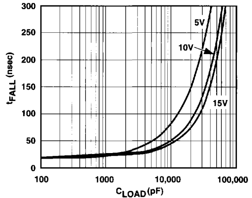
Fall Time vs. Capacitive Load
