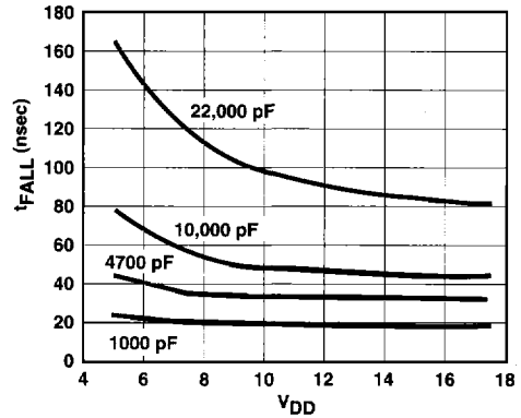
Fall Time vs. Supply Voltage
