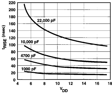
Rise Time vs. Capacitive Load
