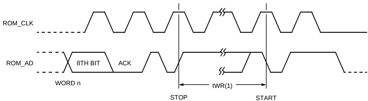
Figure 8. Bus Timing
