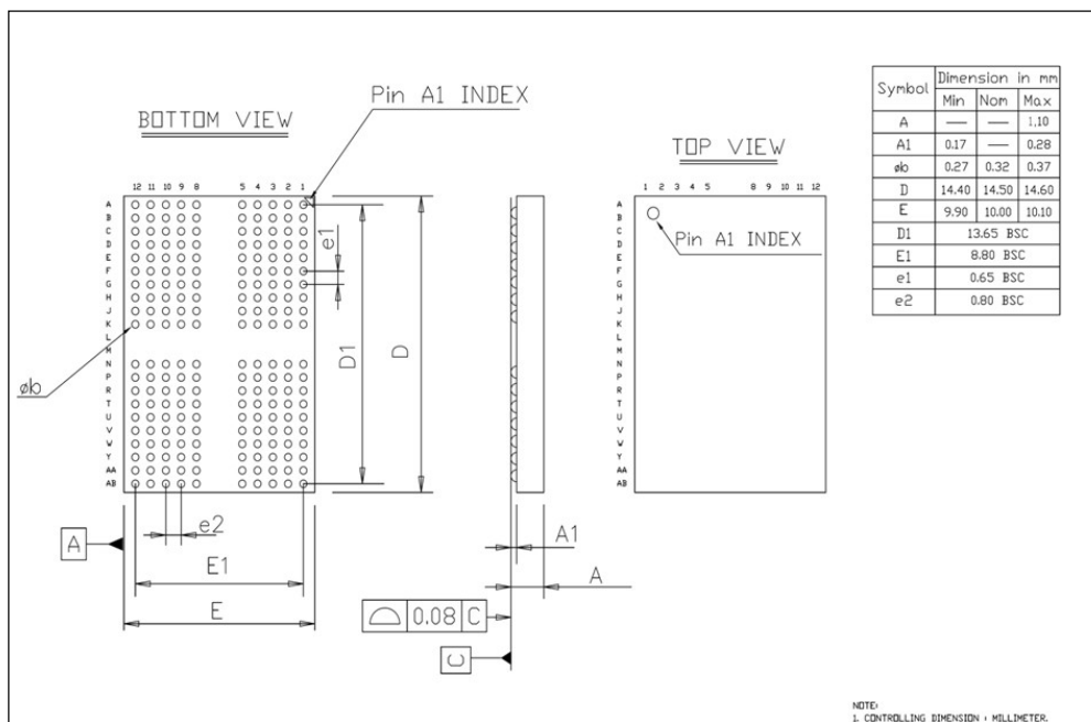
Figure 4 - Package Outline
