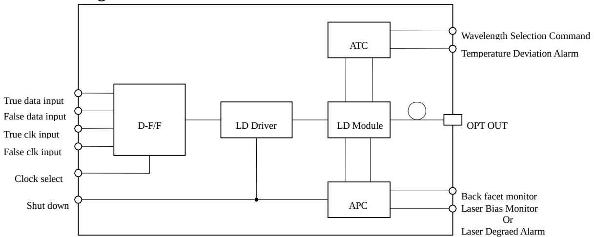
Figure 2.1 Block Diagram
