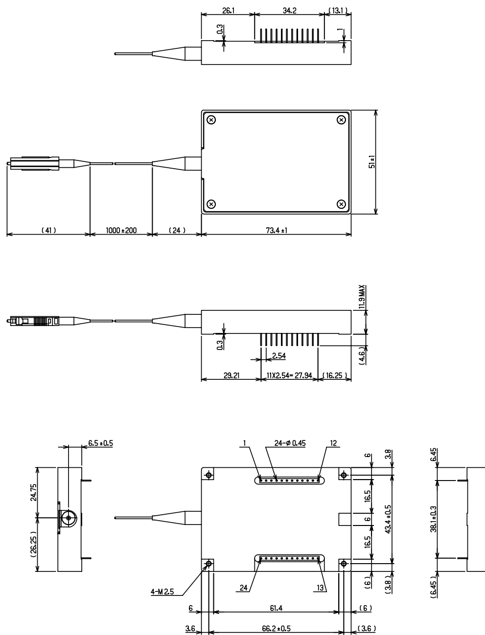
Figure 2.2 Package Outline
