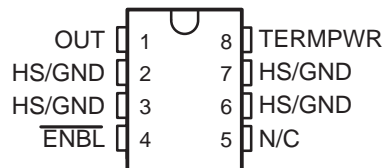
DP PACKAGE (TOP VIEW)
