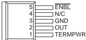
TO-263-5 T PACKAGE (FRONT VIEW)
