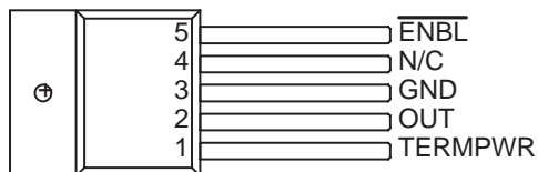
TO-220-5 TD PACKAGE (FRONT VIEW)
