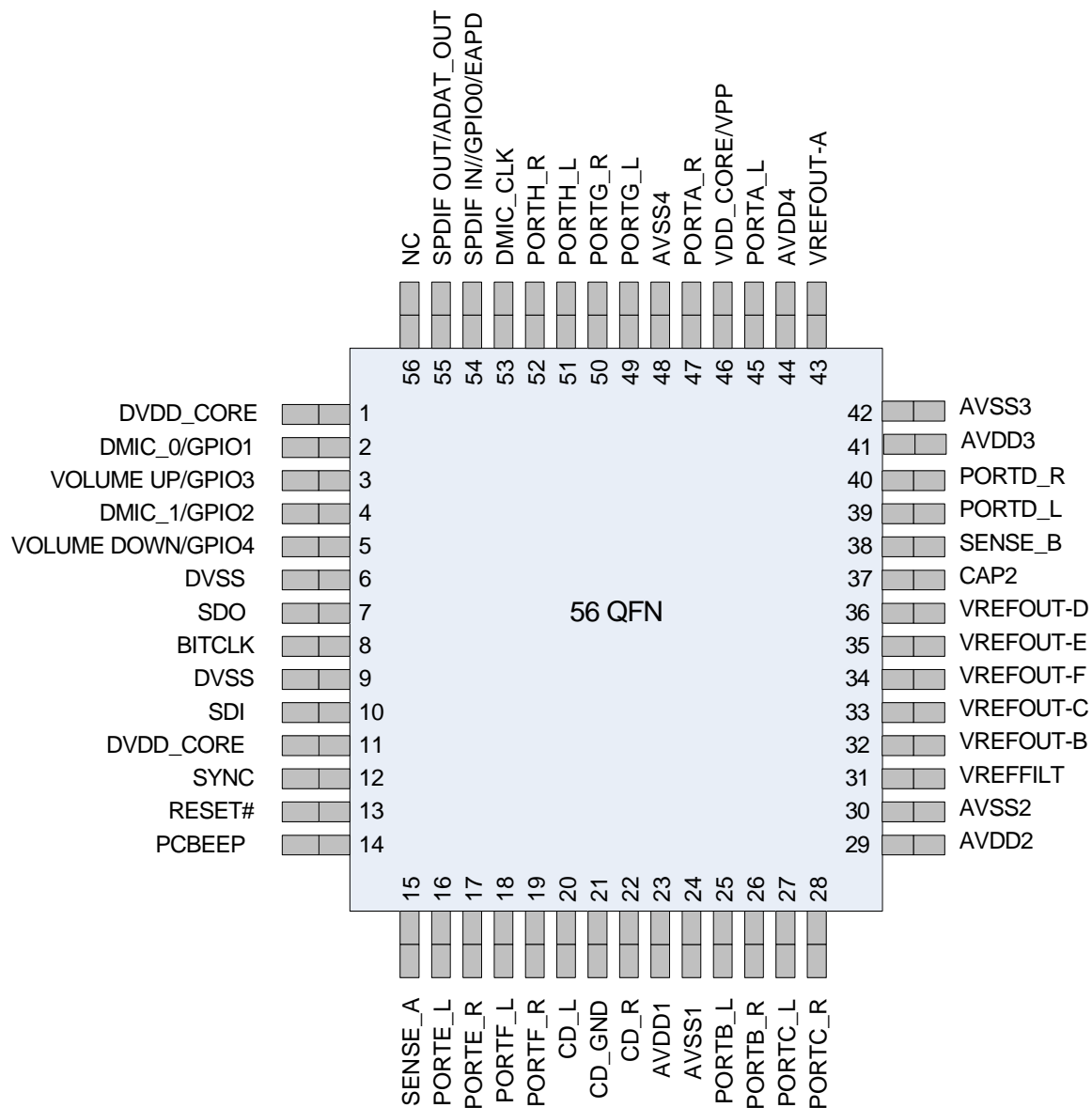
Figure 5. 56-Pad QFN Pinout
