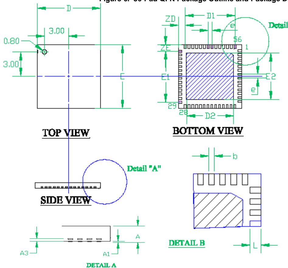
Figure 6. 56-Pad QFN Package Outline and Package Dimensions
