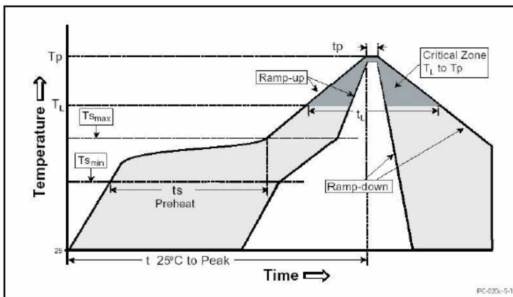
Figure 8. Solder Reflow Profile
