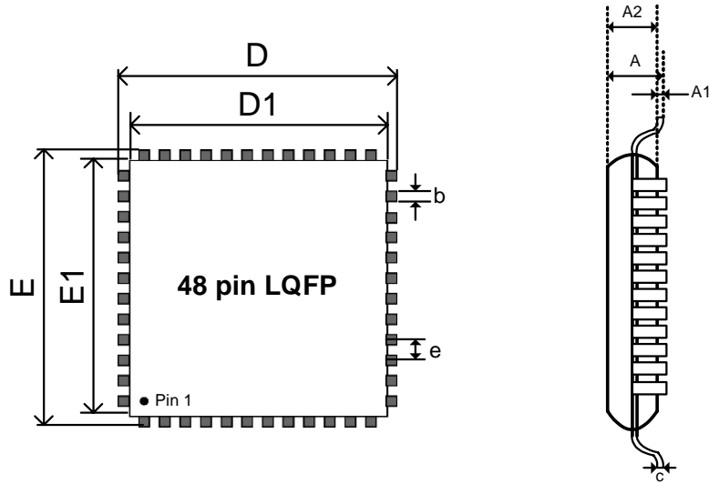
Figure 7. 48-Pin LQFP Package Outline and Package Dimensions
