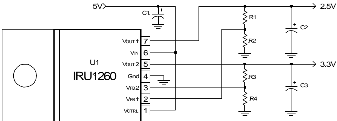
Figure 6 - Typical application of IRU1260 in the Rambus™ design with the 2.5V output providing for memory termination while 3.3V supplies the on board logic.
