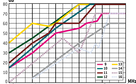
Attenuation Curves on 50Ω MIL STD - 220
