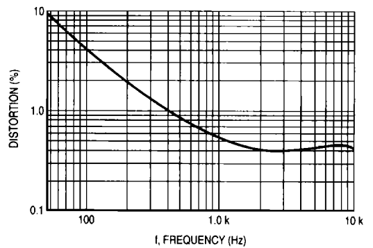
Figure 5. Single Channel Distortion at 50% Modulation
