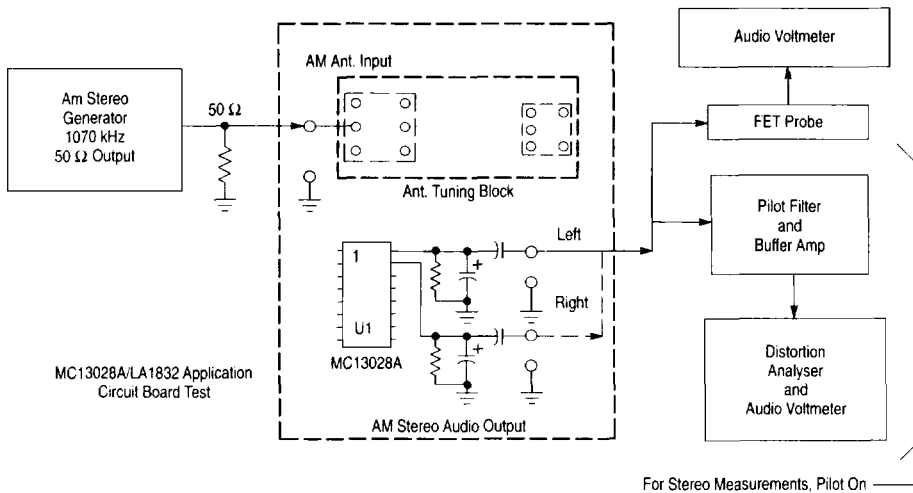
Figure 22. MC13028A/LA1832 Application Circuit Board Test Set-up
