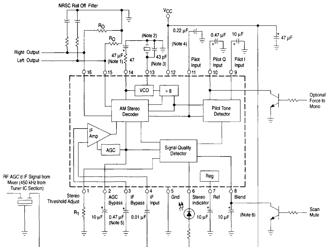
Figure 1. Typical Circuit for E.T.R. Applications
