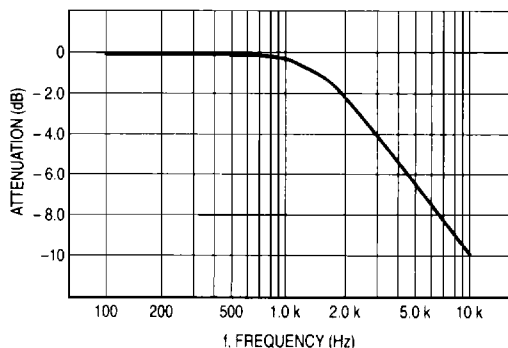
Figure 20. NRSC De-Emphasis Curve for the United States
