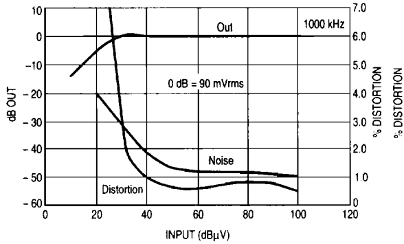
Figure 23. Left AM Output at 30% Modulation
