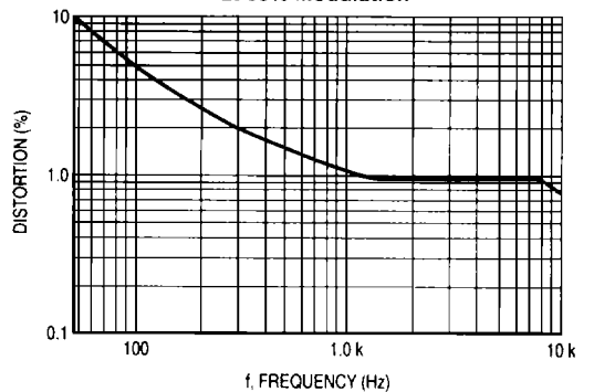
Figure 7. Single Channel Distortion at 65% Modulation
