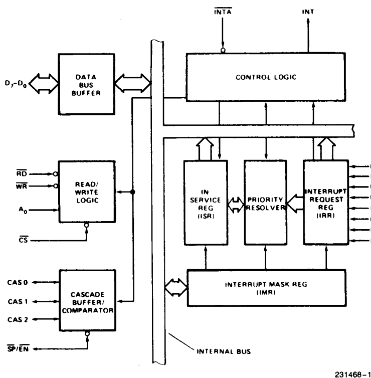
Figure 1. Block Diagram
