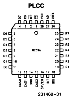
Figure 2. Pin Configurations
