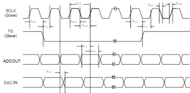
Figure 33: Digital Audio Interface Slave Mode Timing
