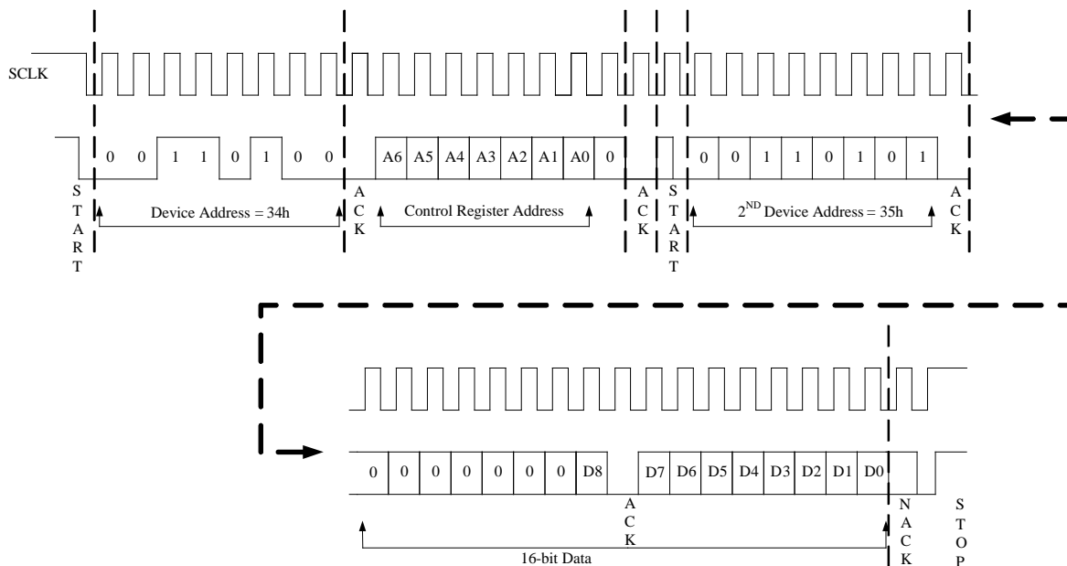
Figure 20: Read Sequence
