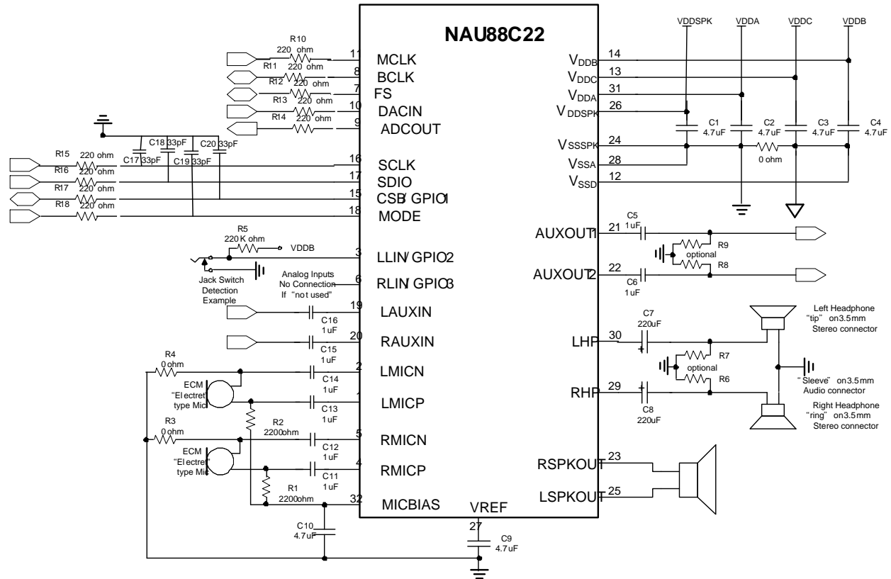
Figure 36: Schematic with recommended external components for typical application with AC-coupled headphones and stereo electret (ECM) style microphones.
