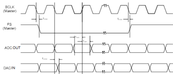
Figure 34: Digital Audio Interface Master Mode Timing
