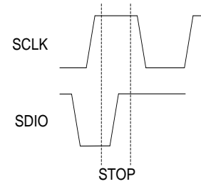
Figure 17: Valid STOP Condition
