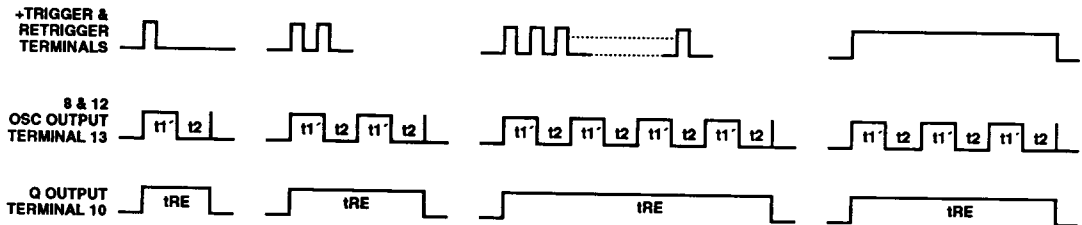
FIGURE 31. RETRIGGER MODE WAVEFORMS
