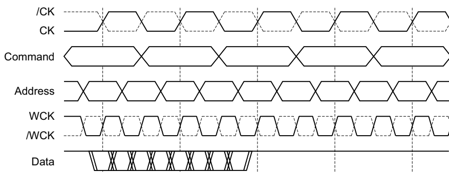
Figure 1: GDDR5 Clocking and Interface Relationship
