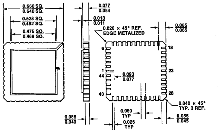
44-Pin Ceramic Leadless Chip Carrier (LCC)
