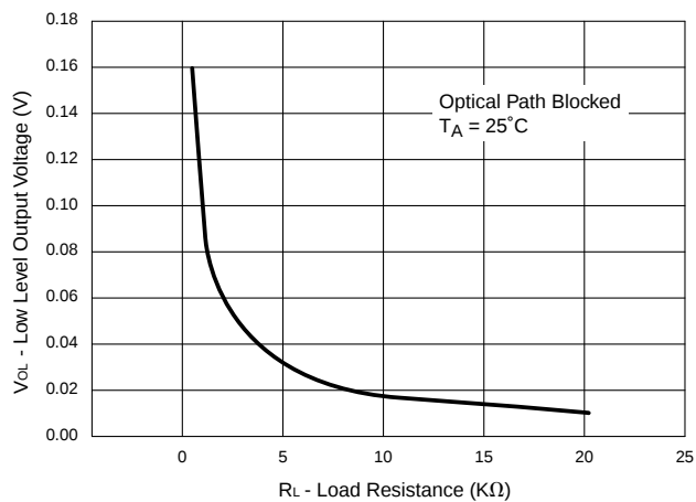
Fig. 6 Low Level Output Voltage vs. Load Resistance
