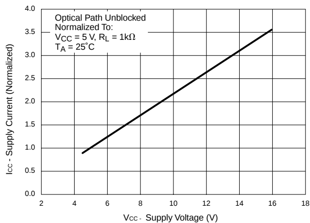
Fig. 4 Supply Current vs. Supply Voltage
