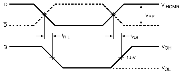
FIGURE 1. Differential PECL to TTL Output Propagation Delay
