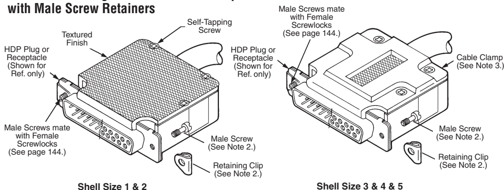
Shell Size 1 & 2
