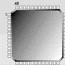
48 Lead LQFP
