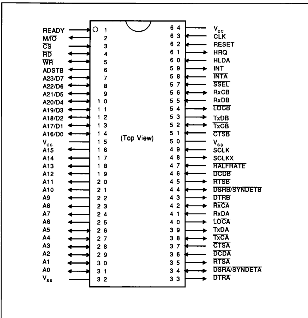
Figure 1-2. Pin Assignment (64-pin SH-DIP)
