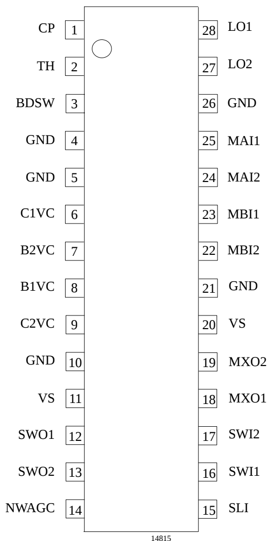
Figure 2. Pinning
