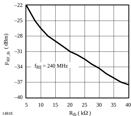
Figure 5. RF power adjustment by R_{\text{th}}
