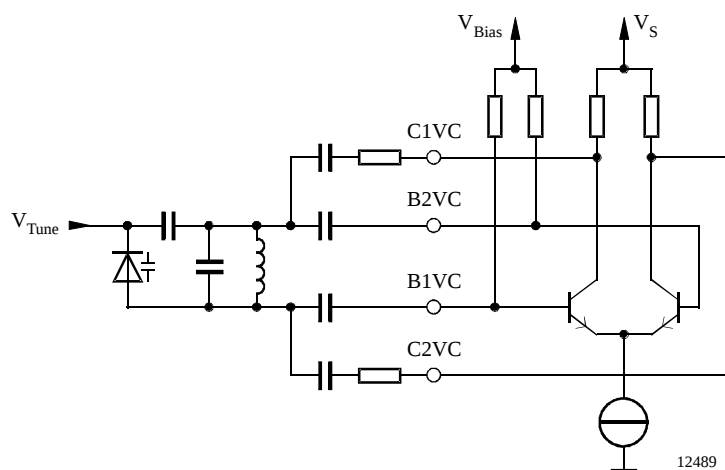
Figure 9. VCO circuit
