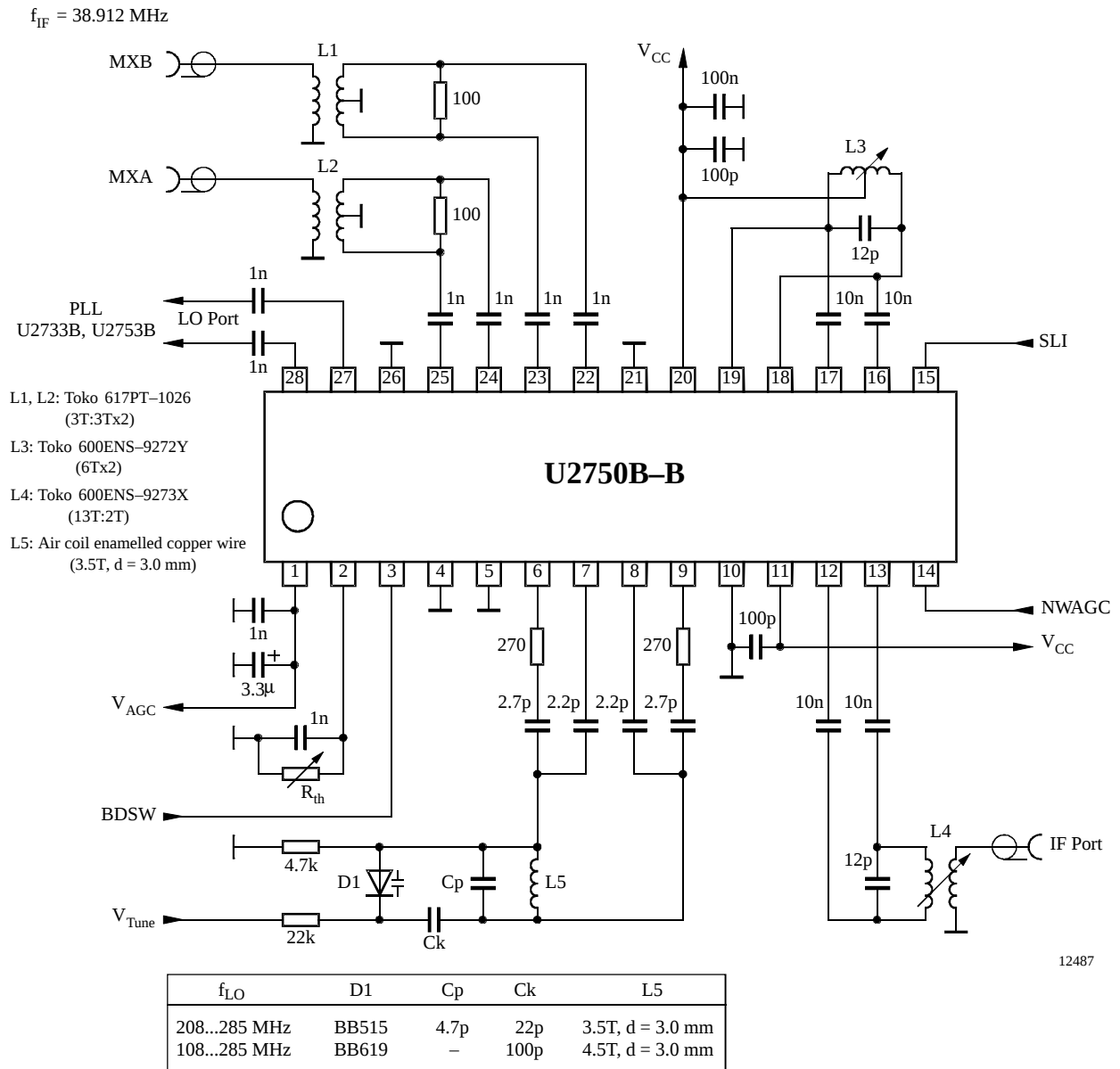
Figure 7. Application circuit
