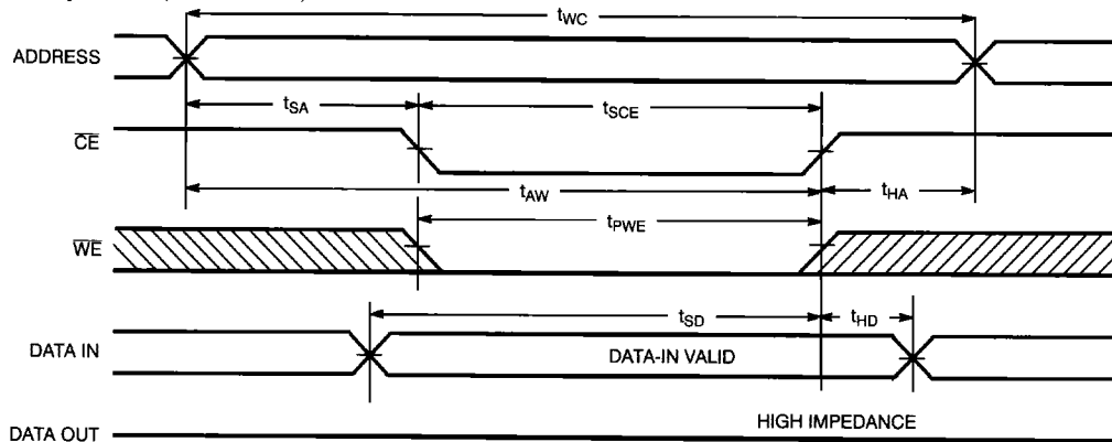
Write Cycle No. 2 ( \overline{CE} Controlled) [9, 13, 14, 16]
