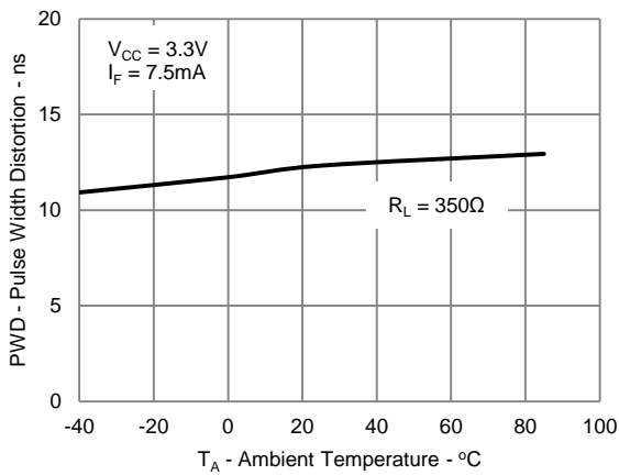
Figure 10: Typical Pulse Width Distortion vs. Ambient Temperature
