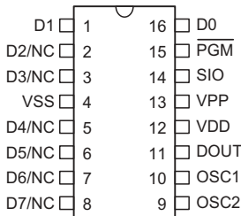
HT6P20 - 16 DIP/NSOP
