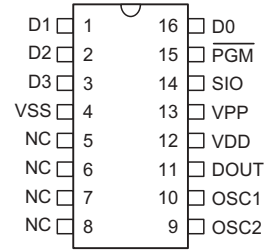
HT6P20D - 16 DIP/NSOP
