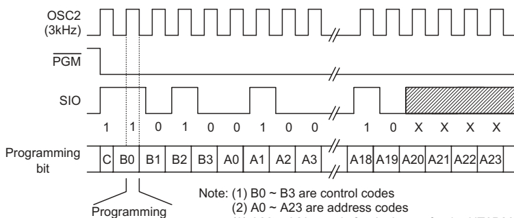
Programming timing for the HT6P20D
