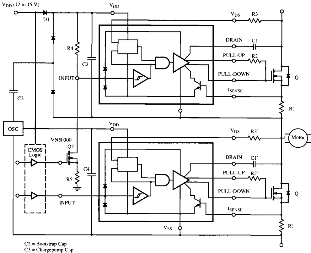
Figure 1. High-Voltage Half-Bridge with Si9910 Drivers
