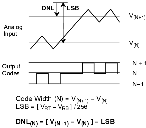
Figure 2. DNL Measurement
