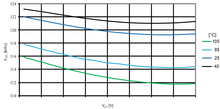
Figure 30-39. Calibrated 8MHz RC Oscillator vs. V CC
