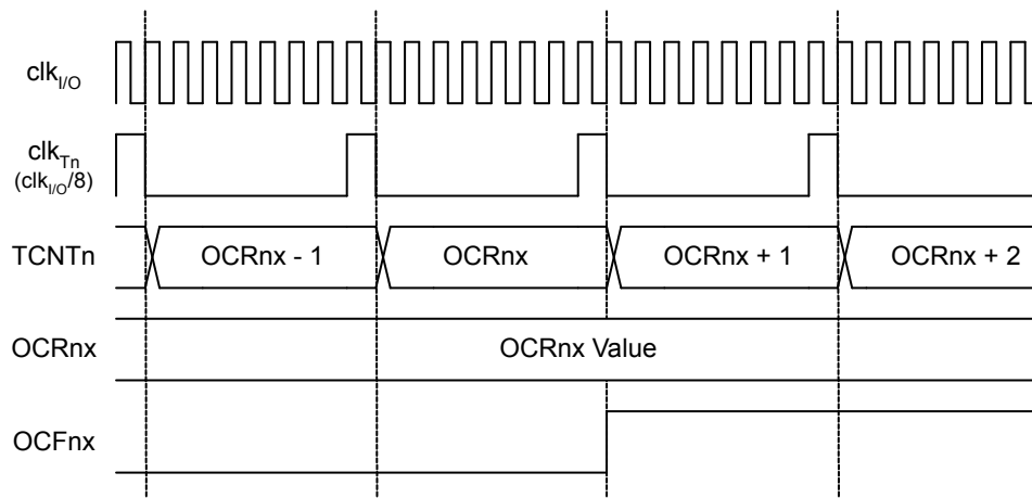
Figure 17-12. Timer/Counter Timing Diagram, Setting of OCF1x, with Prescaler ( f_{\text{clk}_{I/O}/8} )
