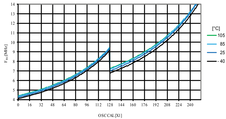
Figure 30-41. Calibrated 8MHz RC Oscillator vs. OSCCAL Value
