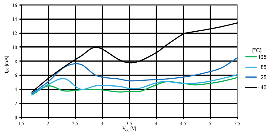
Figure 30-47. Watchdog Timer Current vs. V_{CC}
