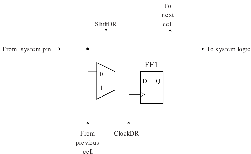
Figure 26-7. Observe-only Cell
